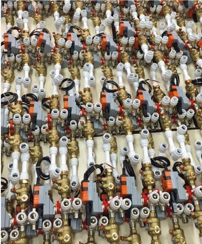
Assembly manufactured in small series, consisting of a 6-way valve, a PIQCV and pipe parts, bends and connections. Pressure-independent solution for the 4-pipe system, ready for installation on-site.
