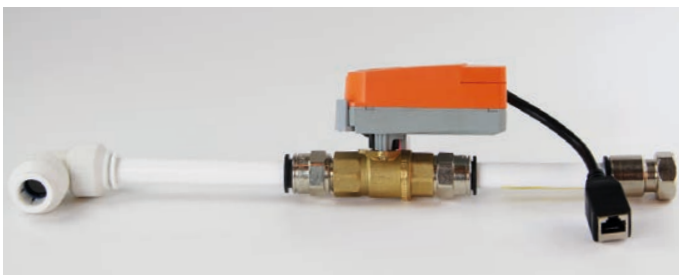
Characterised control valve with pipe parts, bends and connections with customised RJ45 connector socket for connection to a building management system.
