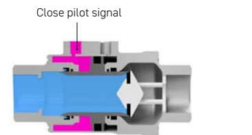
Piloted state (valve closed)
