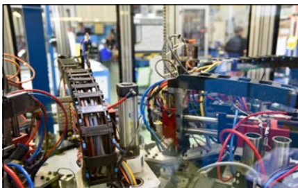
Numerous configurations to optimise pneumatic automation circuits
